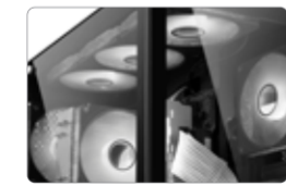
Top fans Mount 3 120mm fans or 2 140mm fans on the top, fix the fans with screws at the anchor points.
